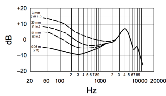
Frequency Response
