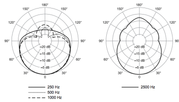
Polar Pattern
