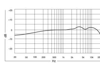
Frequency response
