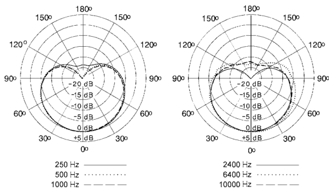
Polar pattern
