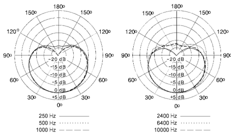
Polar pattern
