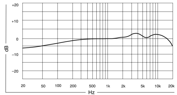
Frequency response
