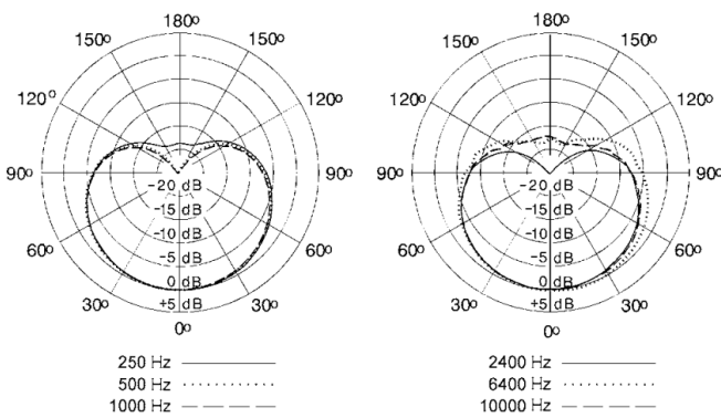
Polar pattern
