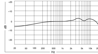
Frequency response
