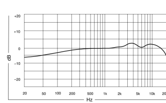
Frequency response
